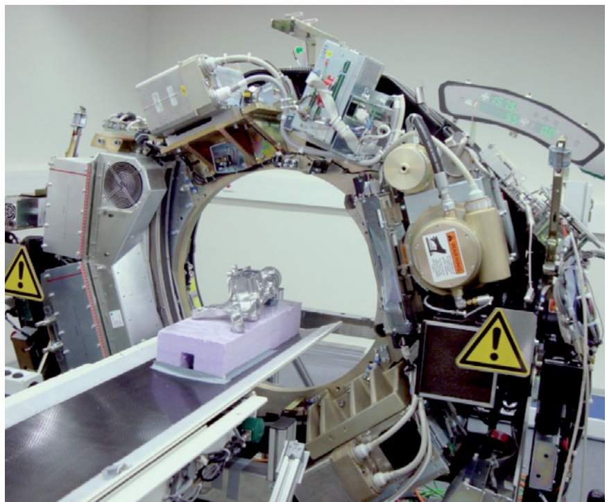
Figure 2. Laboratory-scale high-speed CT scanning a die casting
