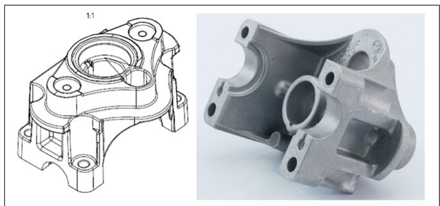
Figure 4: The scanned aluminium die casting
