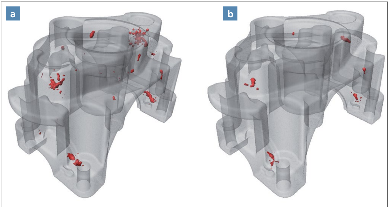
Figure 7: Transparent 3-D model of the test pieces: a) with the highest degree of porosity (part No. 4) and b) with the lowest degree of porosity (part No. 10)
