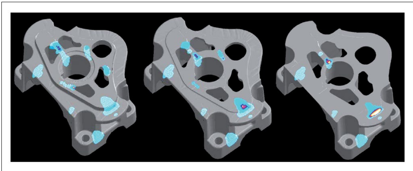
Figure 6: Simulation of the test piece visualizing porosity in different planes of the part (red: probability of pore formation approx. 50 %, yellow: 75 to 85 % and white 100 %)
