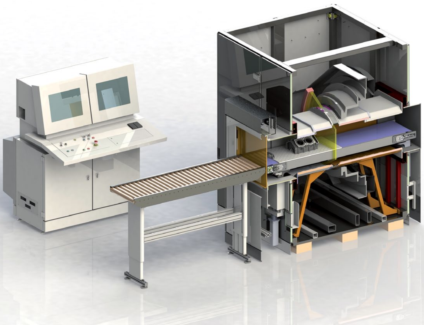
Figure 13: High-speed CT system in at-line arrangement
