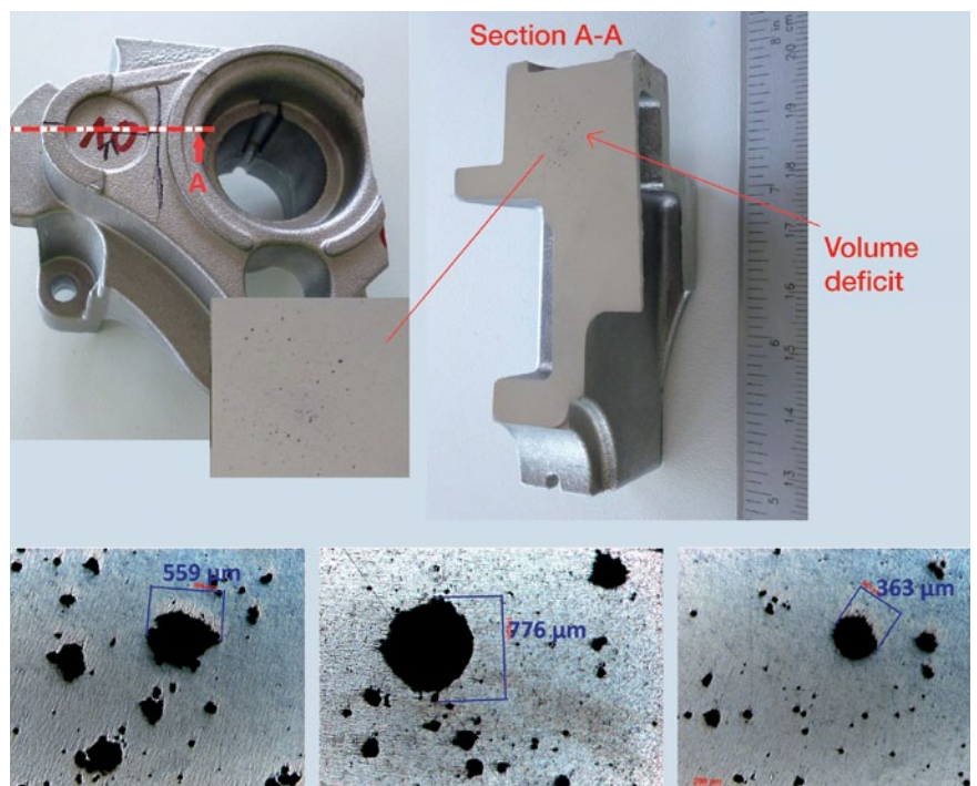
Figure 10: Metallographic examination of part No. 10, the part with the lowest porosity in Figure 7b
