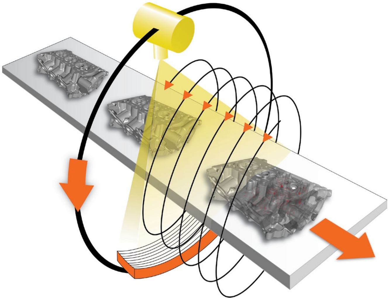
Figure 1: In a high-speed, automatic helix in-line CT unit the gantry, which accommodates the x-ray tube and the multi-line detector arranged opposite, rotates about the specimens on the conveyor belt [6]
