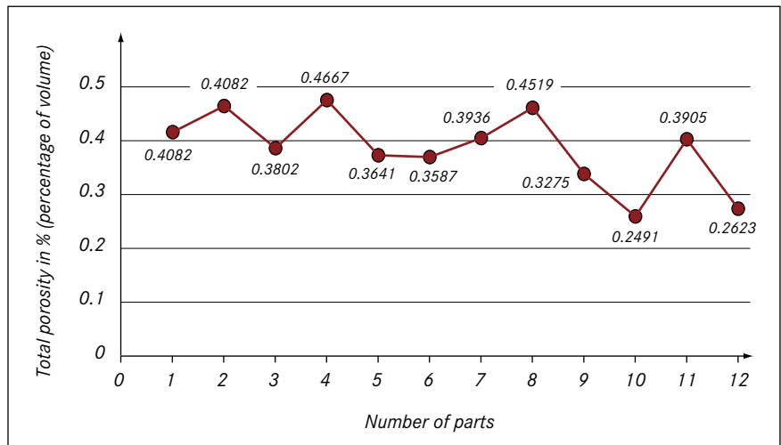
Figure 8: Total porosity relative to number of parts
