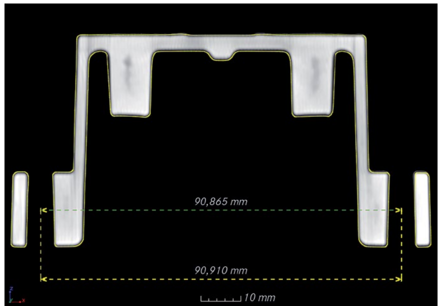
Figure 12: Chosen nominal distance of 91.000 mm measured by high-speed CT and by fringe projection
