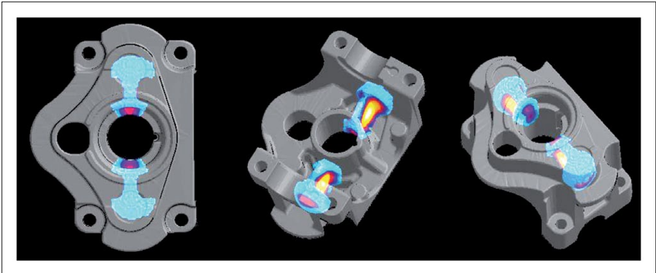
Figure 5: Simulation of the test piece for hot spot identification in different planes of the part (forecast locations of volume deficits due to shrinkage; colour scale: turquoise approx. after 18 s, light red after approx. 20 s, yellow after approx. 21 s)
