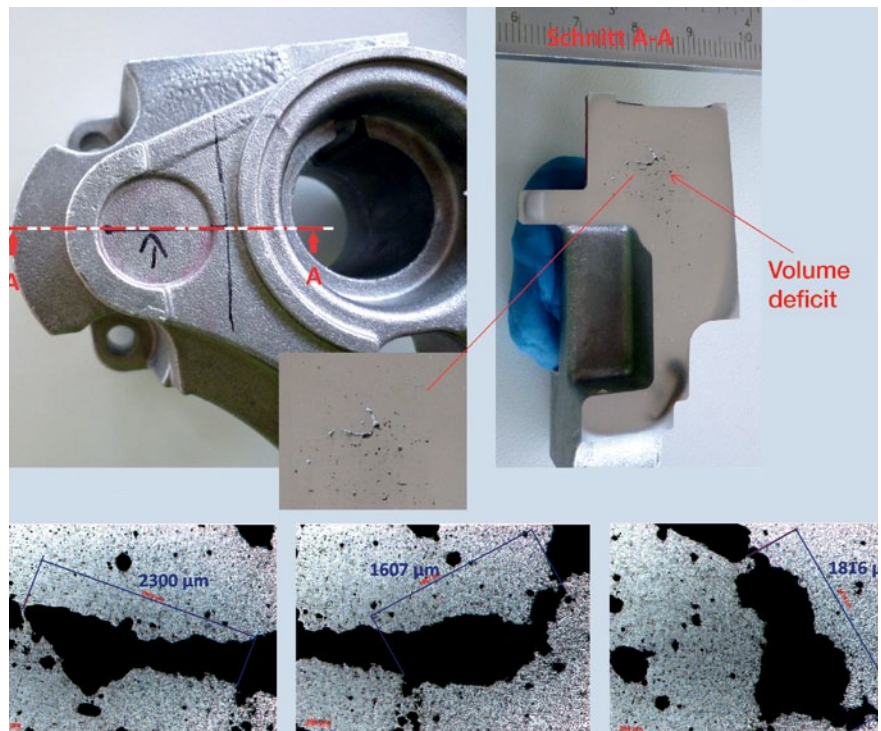
Figure 9: Metallographic examination of part No. 4, the part with the highest porosity in Figure 7a
