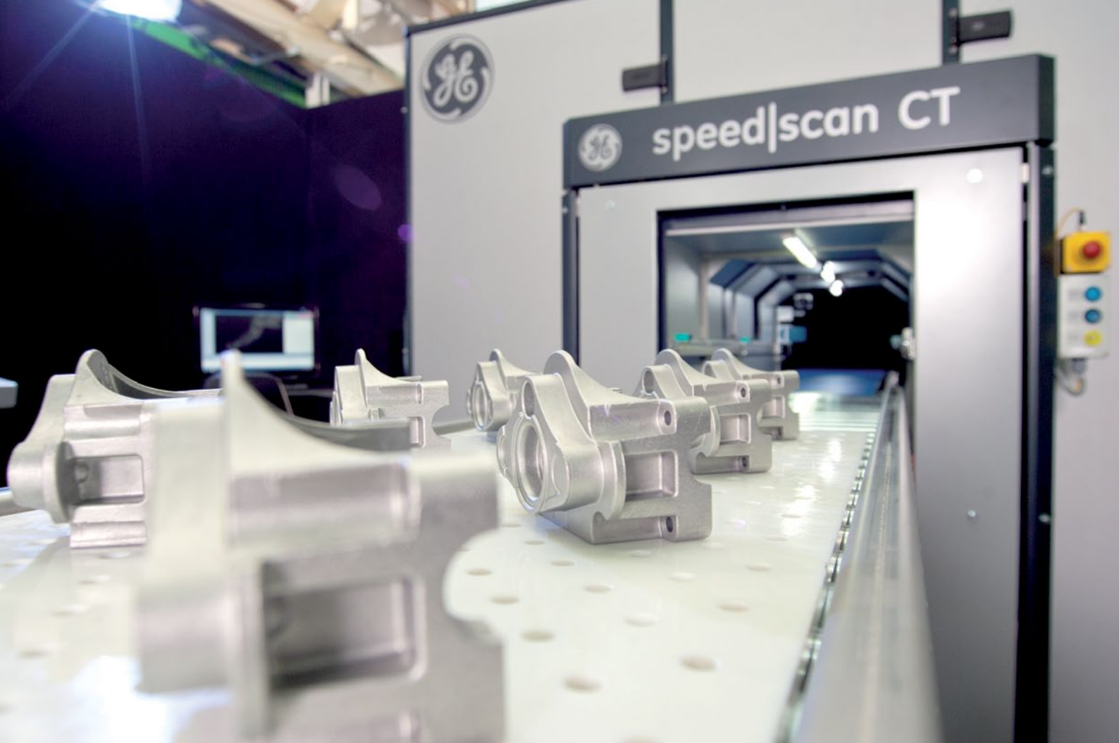
Figure 3: Series-type high-speed CT unit
