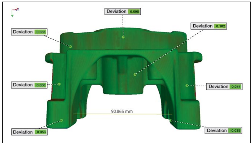
Figure 11: Dimensional deviations of the tomograms versus the fringe-projection-based measurement of part No. 5
